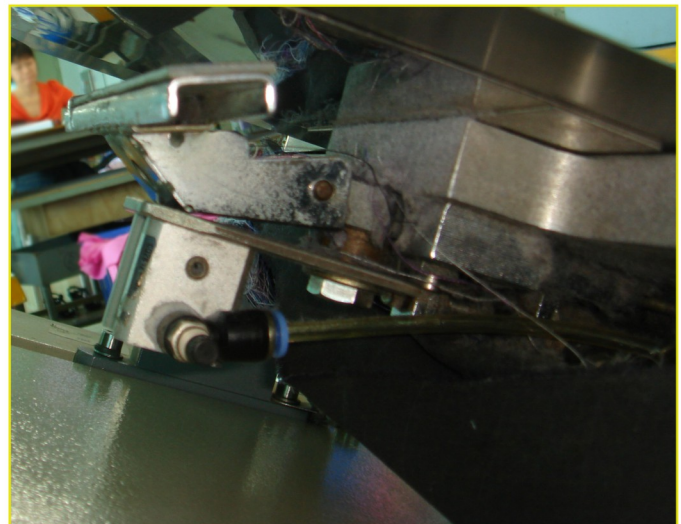
自動底夾，防止操作时袖口移位 Automatic bottom clamp for avoiding cuff shift during operation
