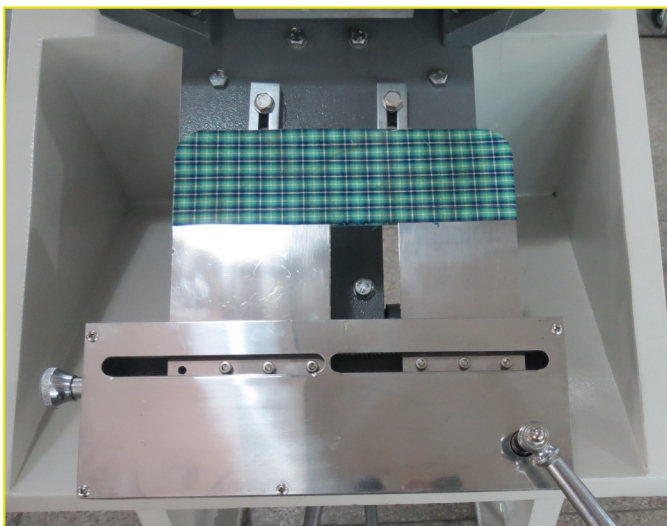
CF-46袖口模板寬度可調 The width of cuff mould can be adjusted
