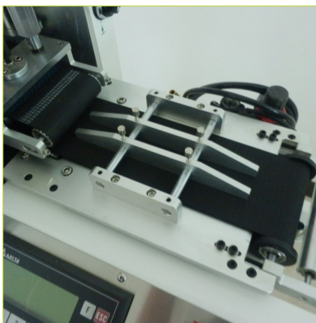
獨特的履帶式送料 Unique crawler type feeding structure
